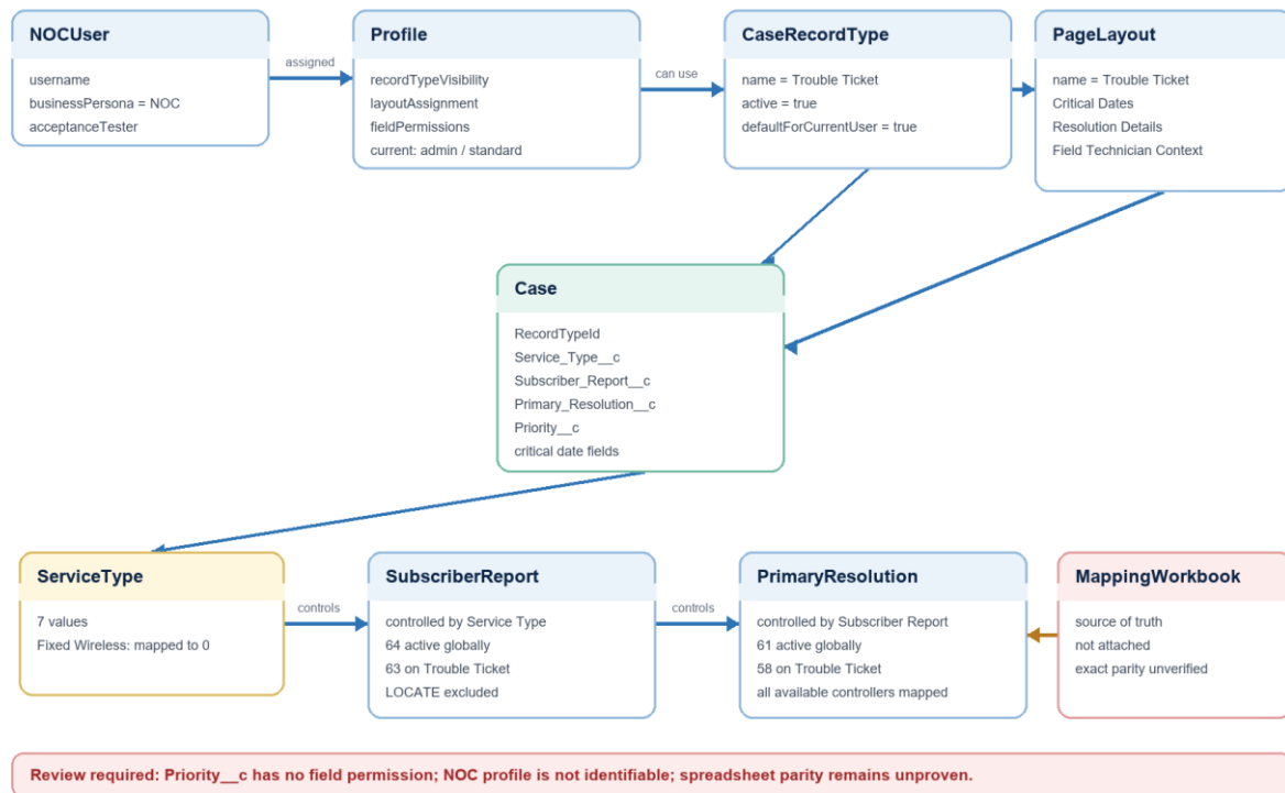
Figure 2. Trouble Ticket configuration and dependency class diagram
